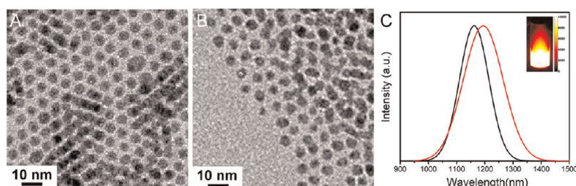
Figure 2. TEM images of DT-Ag 2 S QDs (A) and DHLA-Ag 2 S QDs (B) and their NIR PL spectra (C) (black line: DT-Ag 2 S QDs; red line: DHLA-Ag 2 S QDs). Inset shows a PL image of DHLA-Ag 2 S QDs suspension under an 808 nm excitation.
